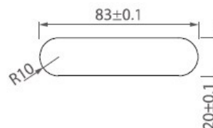
drilling template
